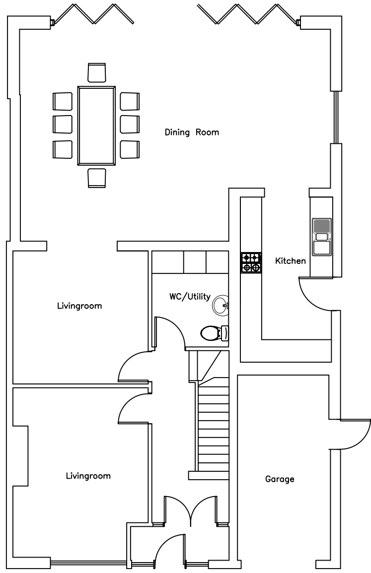
Ground Floor
