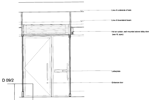
DETAIL SECTION 3 THROUGH LOBBY
