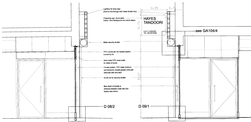
DETAIL SECTION 1 THROUGH FRONTAGE
