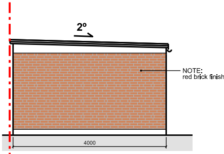
13 OUTBUILDING SIDE ELEVATION 1:100
