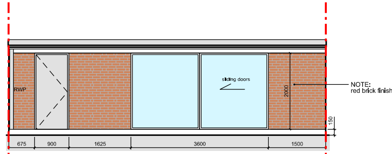
11 OUTBUILDING FRONT ELEVATION 1:100
