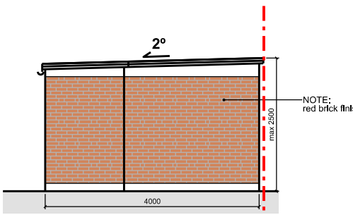
14 OUTBUILDING SIDE ELEVATION 1:100
