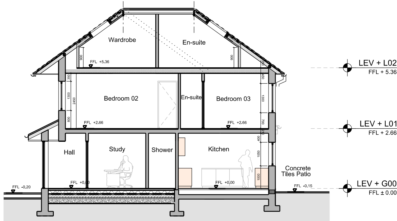
06 SECTION C-C 1:100
