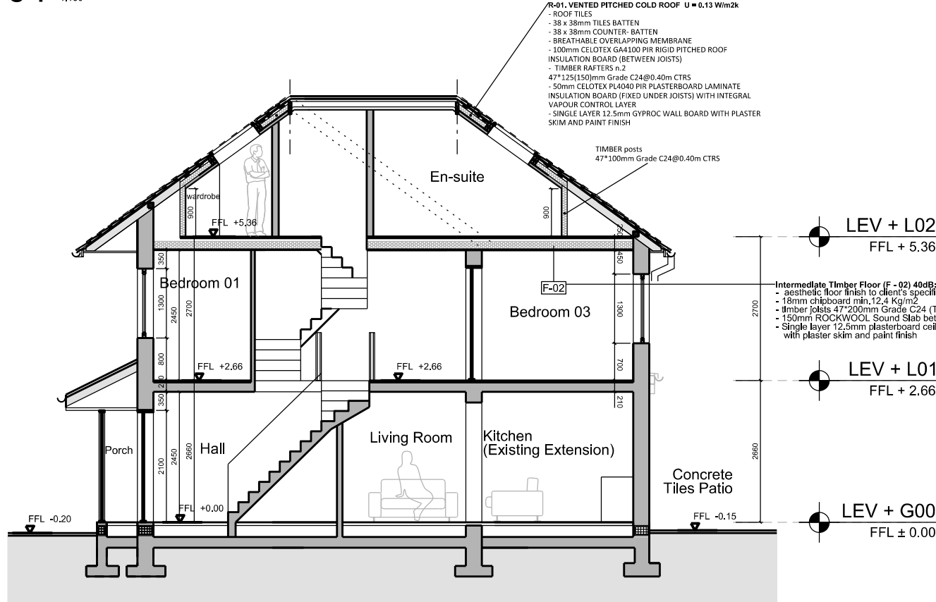
05 SECTION B-B 1:100
