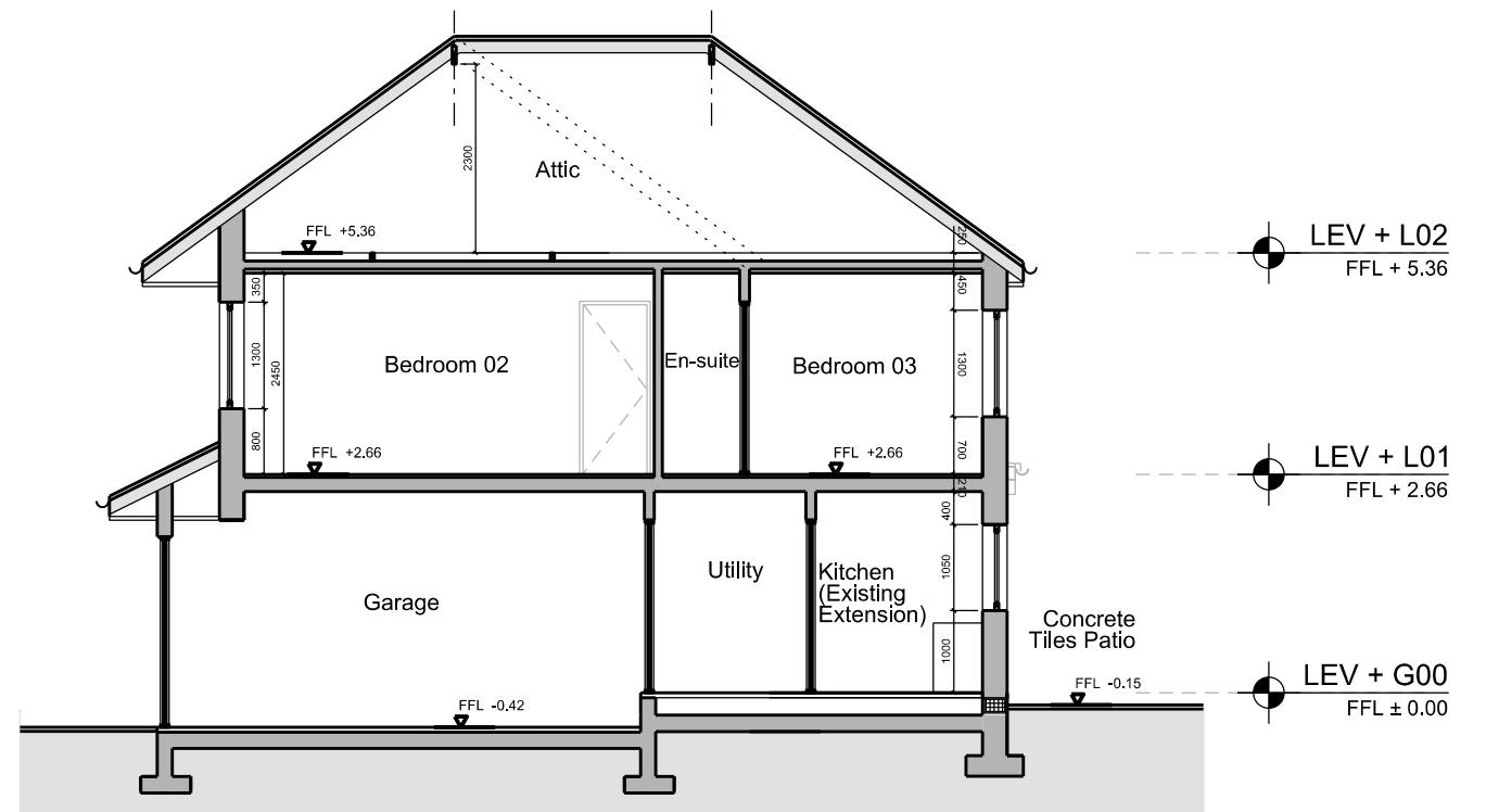
06 SECTION C-C 1:100
