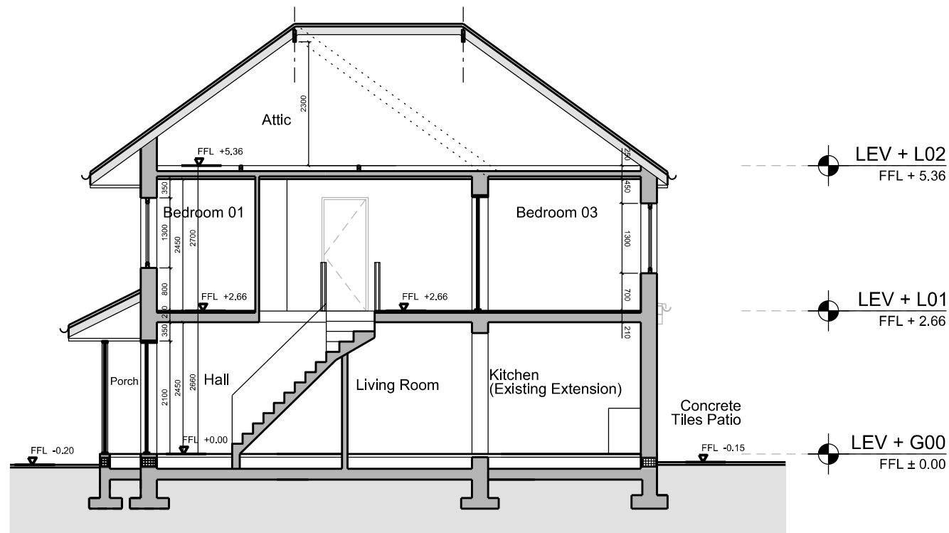
05 SECTION B-B 1:100
