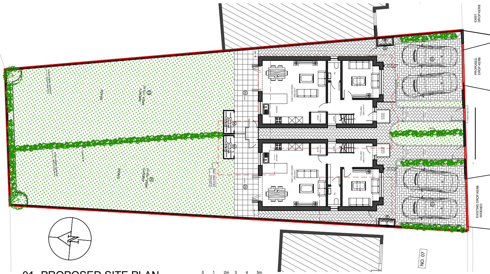
01 - PROPOSED SITE PLAN SCALE 1:200
