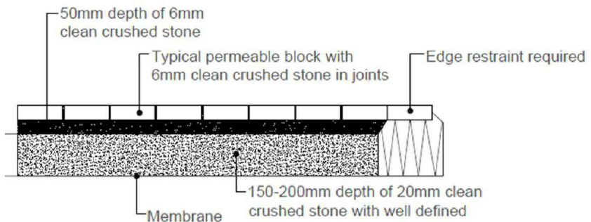
PAVING BUILT-UP DETAIL
