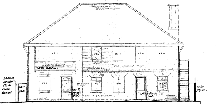
WEST ELEVATION, REAR (MAIN EXISTING BUILDING)
