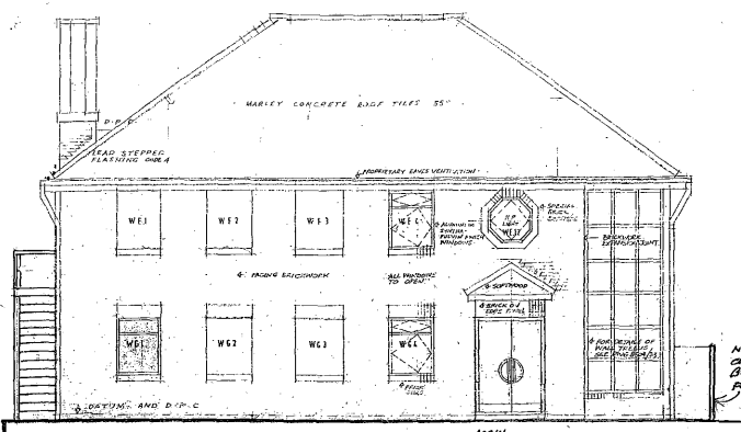
EAST ELEVATION FRONT. (MAIN EXISTING BUILDING)
