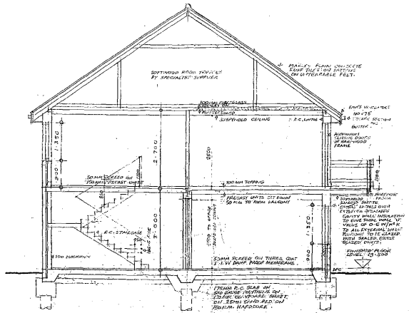
SECTION (MAIN EXISTING BUILDING)
