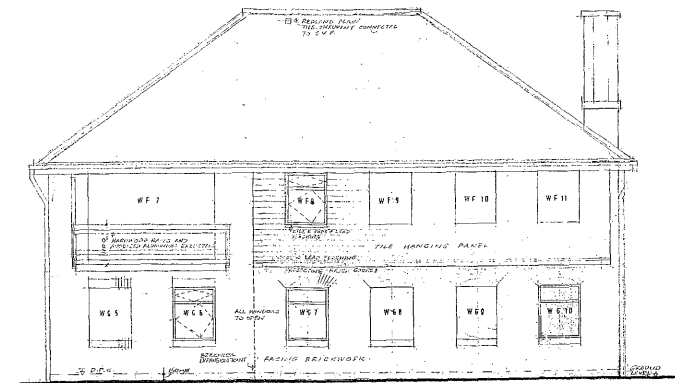
WEST ELEVATION. RISE
