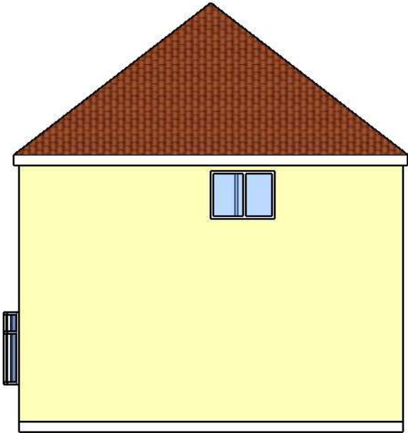
Existing left elevation 1:100
