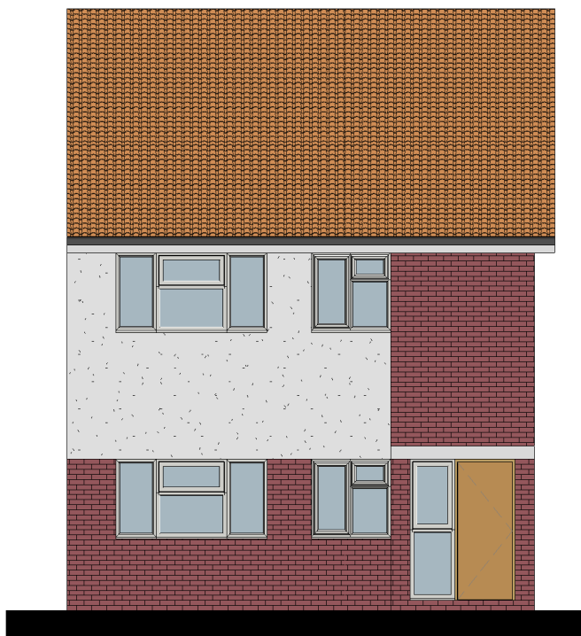
Elevation East Existing 1 : 100
