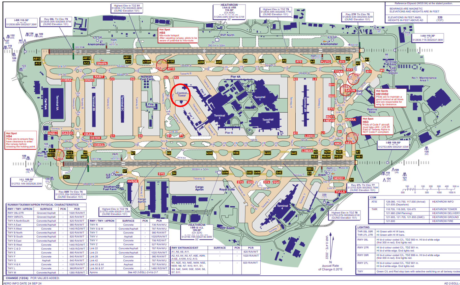
Figure 3 Aerodrome chart for London Heathrow Airport (cropped)
