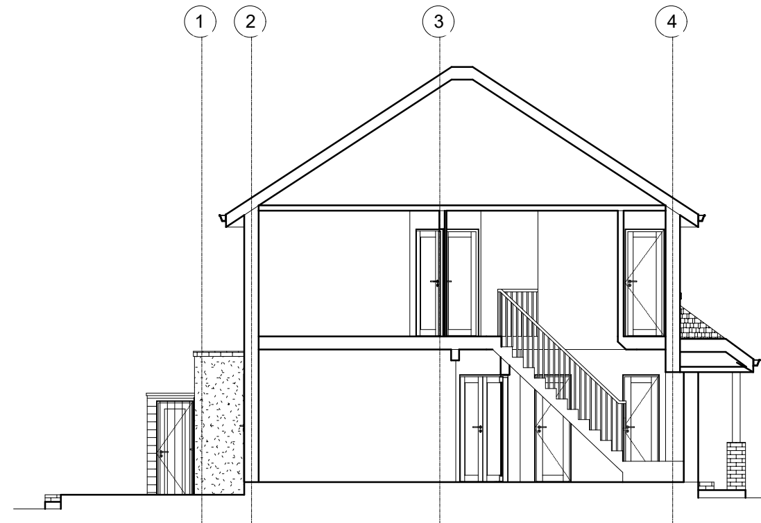
EXISTING SECTION
