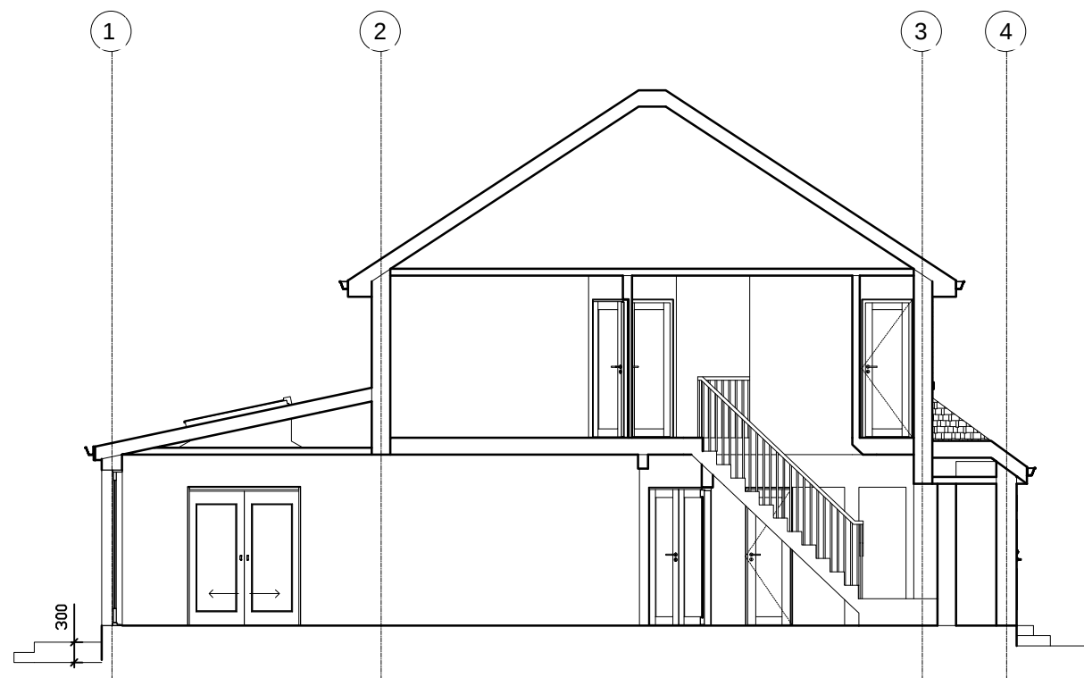
PROPOSED SECTION
