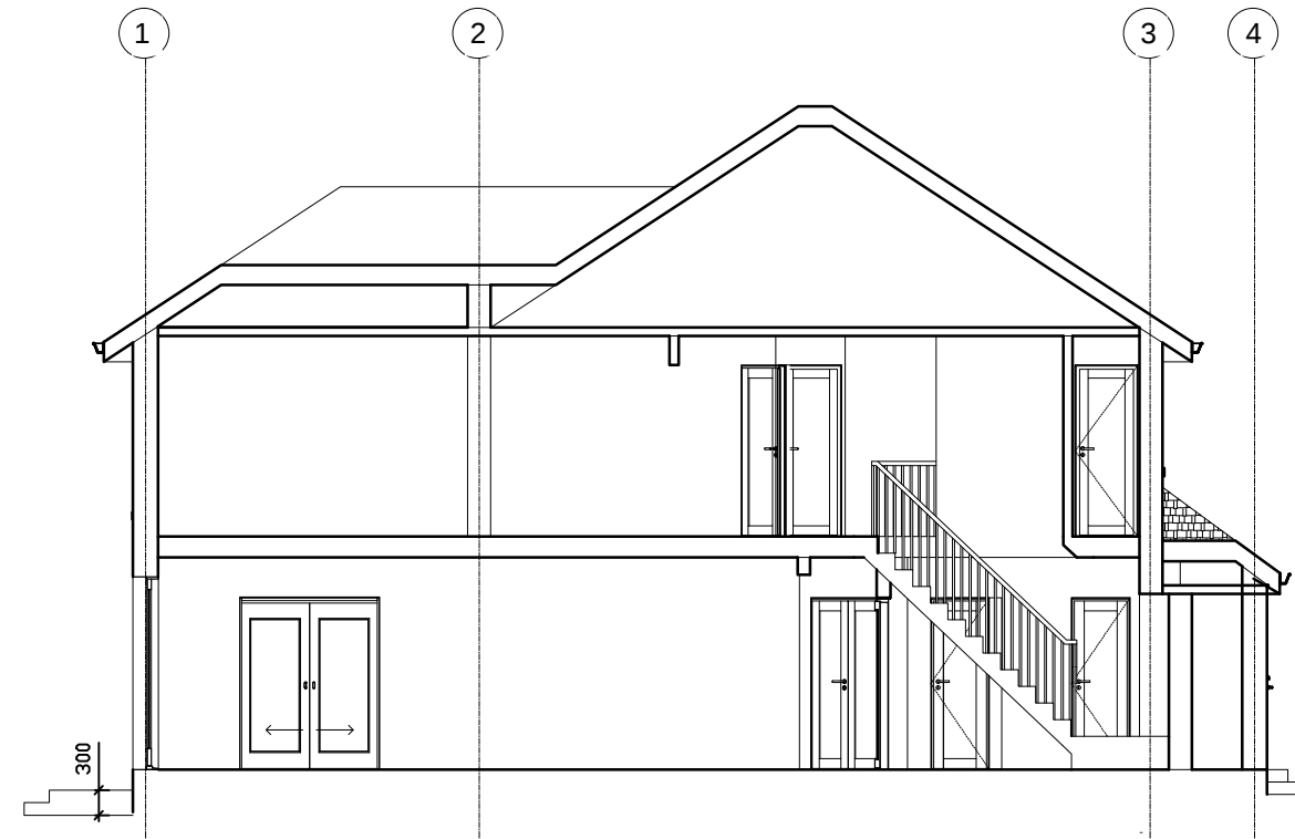
PROPOSED SECTION
