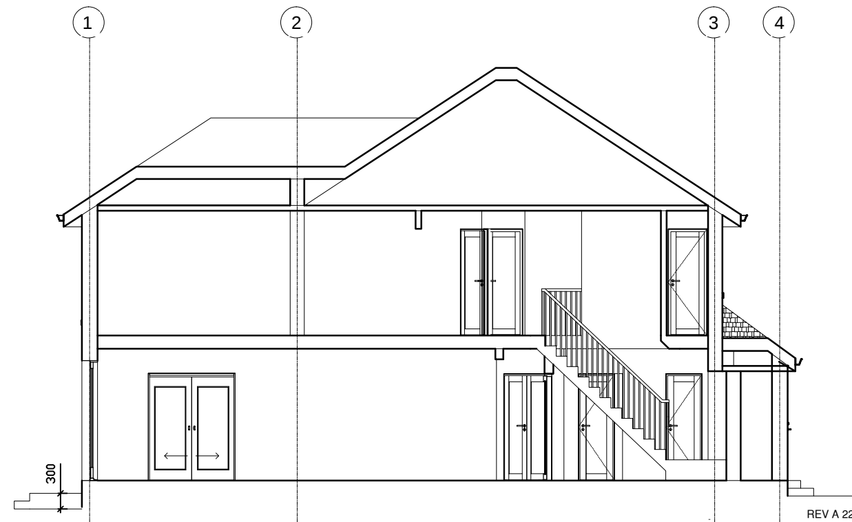
PROPOSED SECTION
