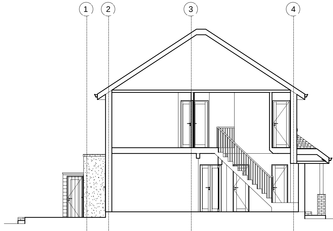
EXISTING SECTION
