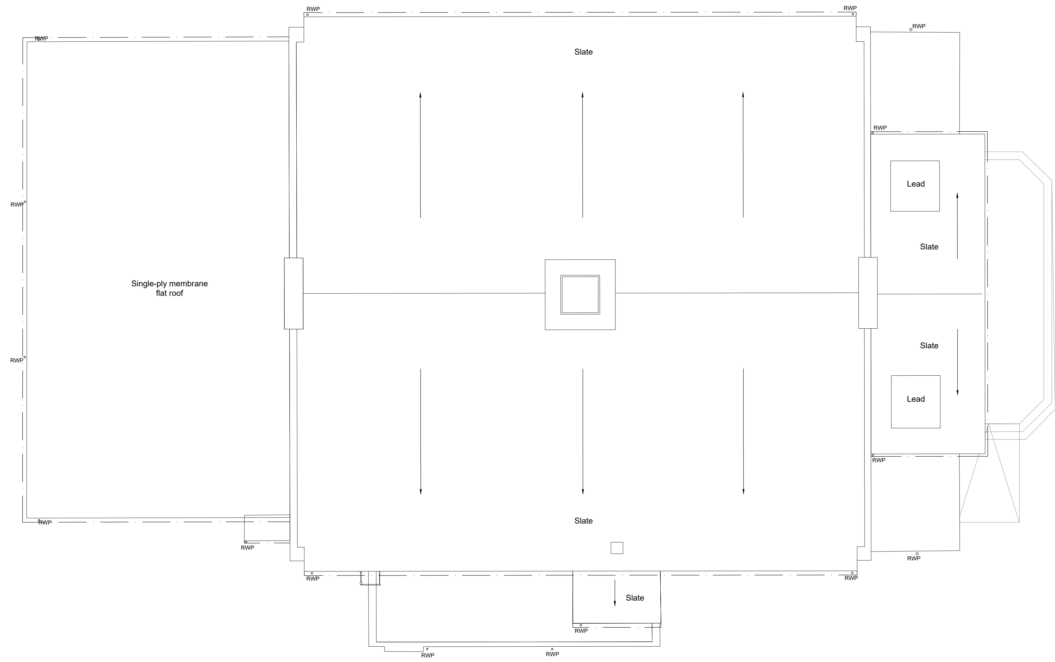
1 Roof Plan - Proposed 2015 1:100
