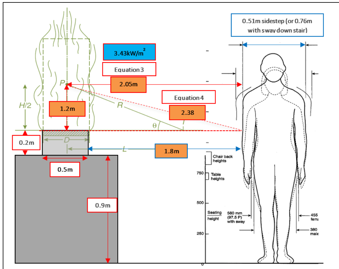
Figure 15 - Notional section through fire scenario
