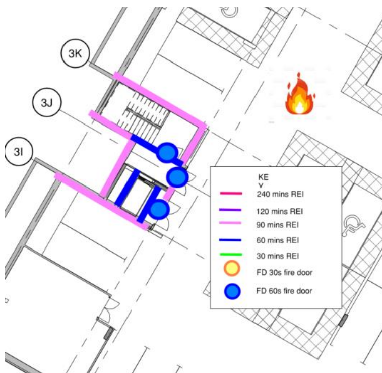
Figure 19 - Fire Scenario in Basement Car Park with Block 3 Design
