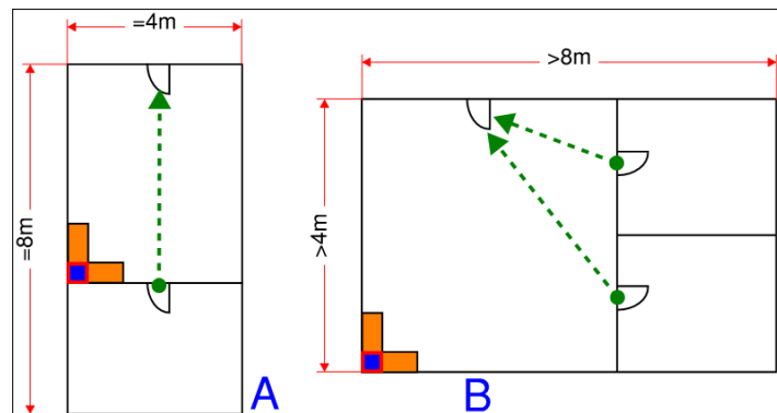
Figure 17 - Various open plan designs for comparison
