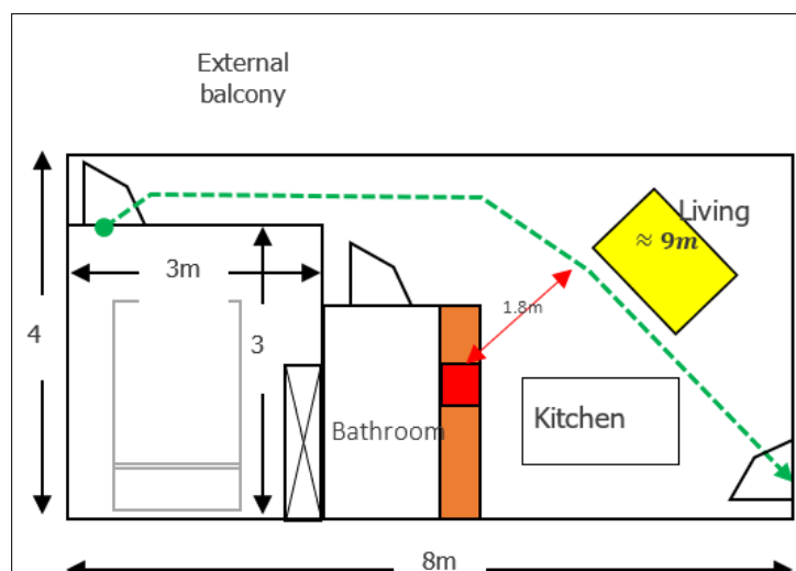
Figure 18 - Code compliant travel distance within an open plan flat with the kitchen open
