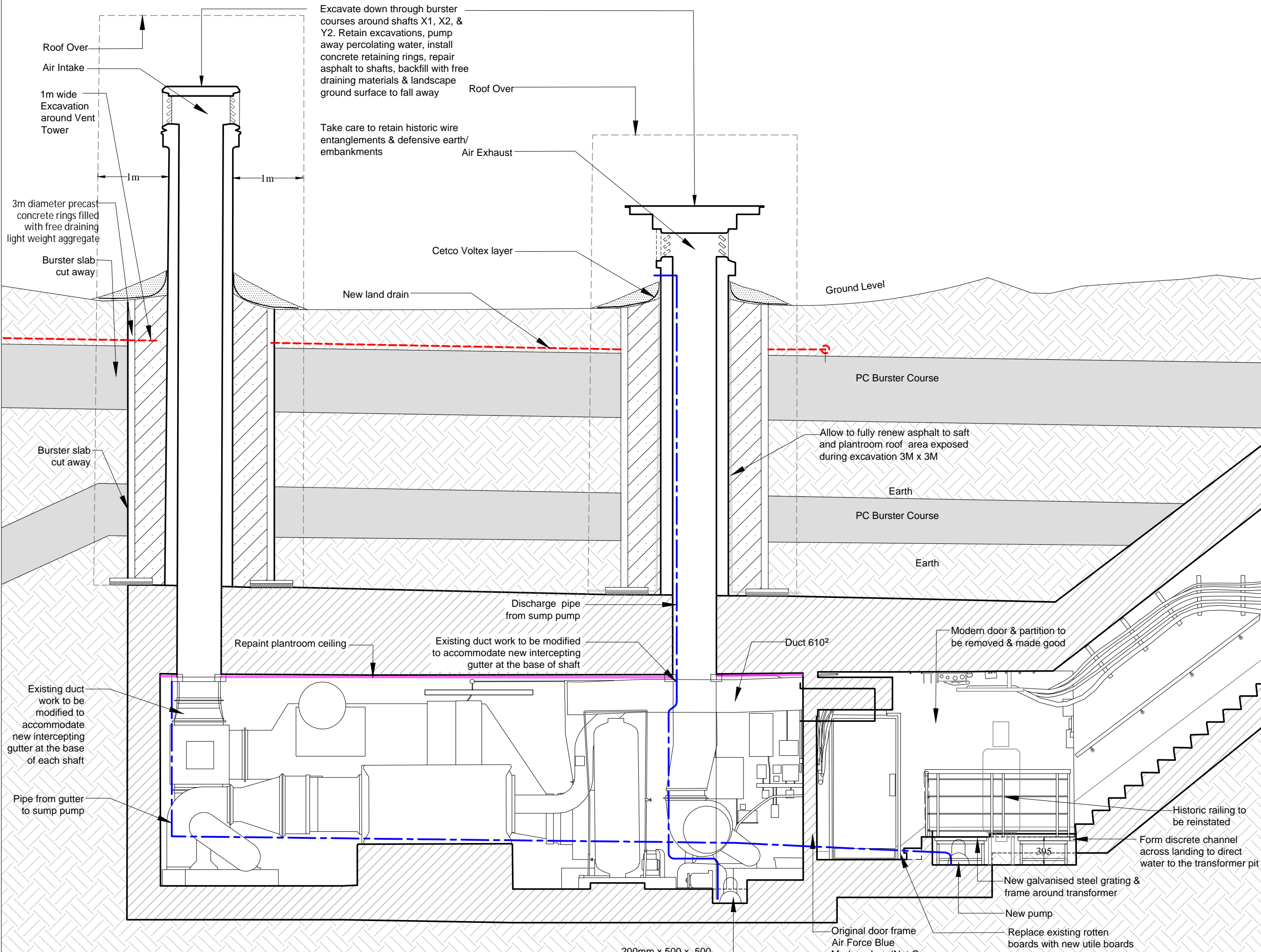
SECTION THROUGH X PLANT ROOM - DETAIL As Proposed, 1:50
