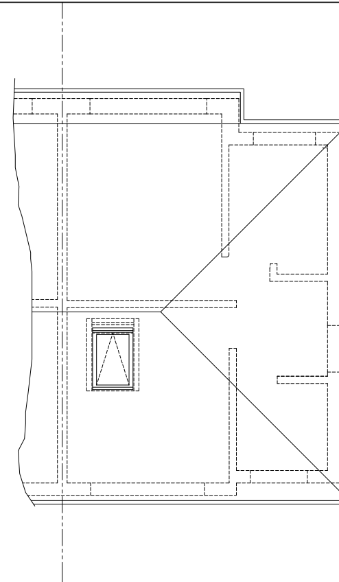
Existing Main Roof Plan
