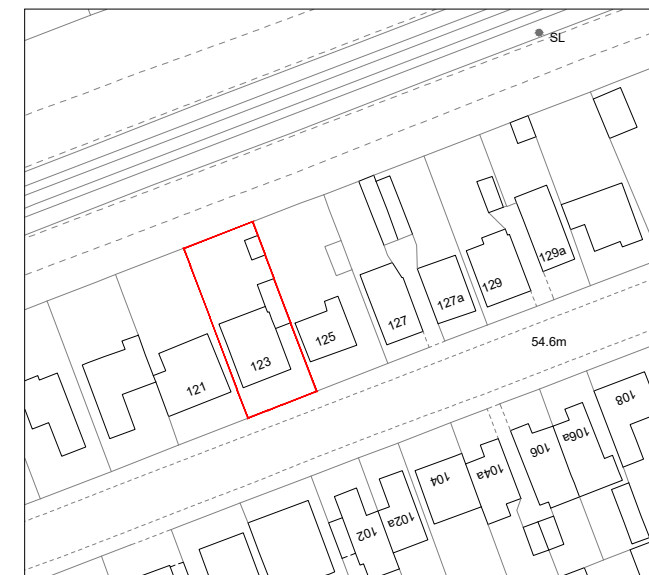
Location plan (1:1250)
