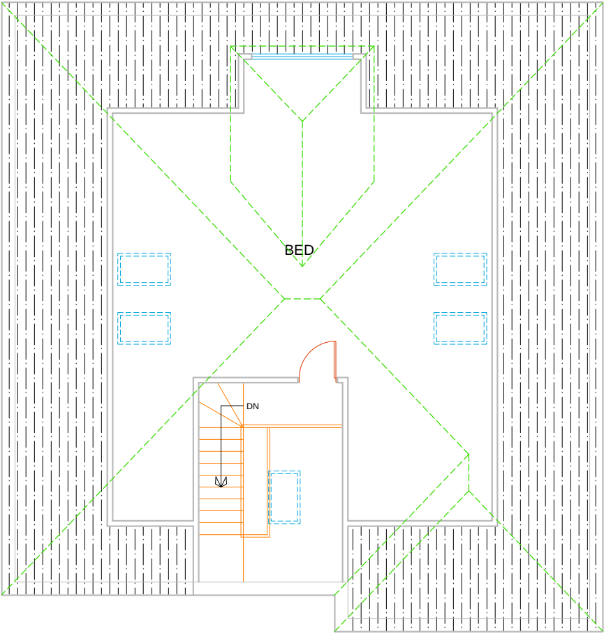
EXISTING LOFT PLAN
