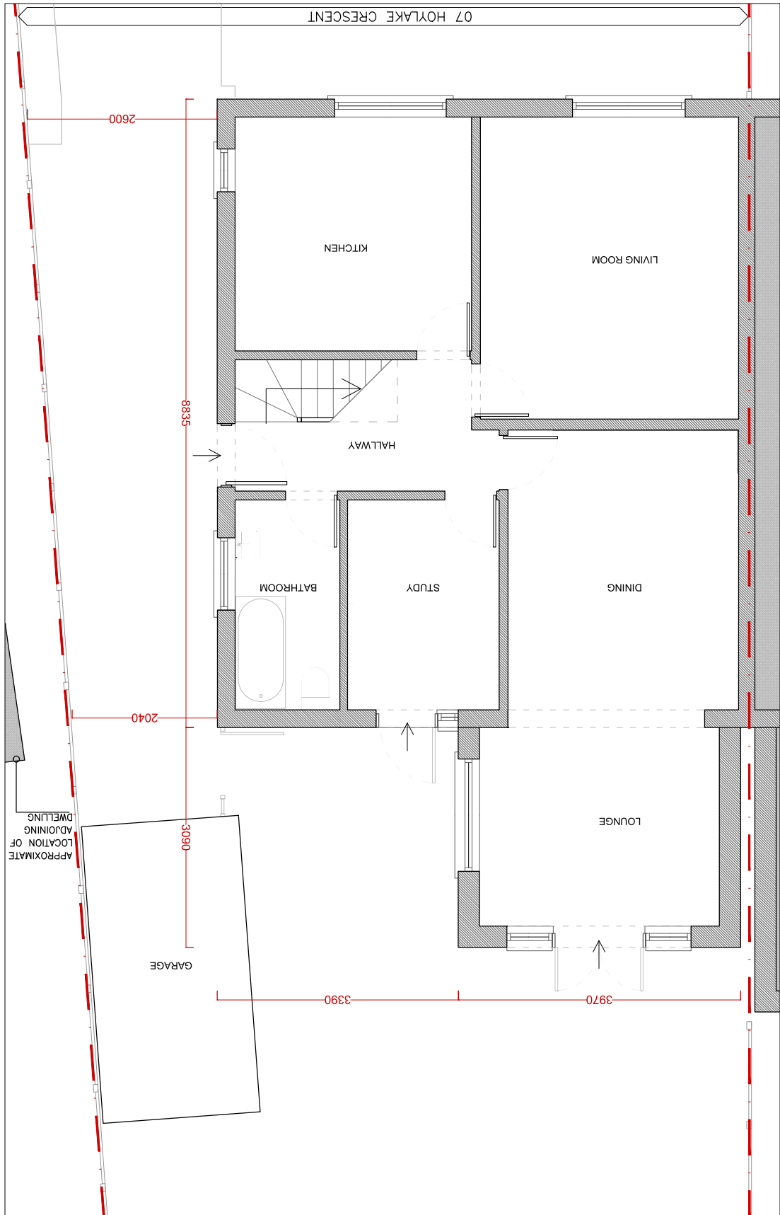
E-05 EXISTING GROUND FLOOR PLAN
