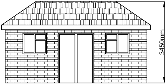
PROPOSED FRONT ELEVATION @1:100
