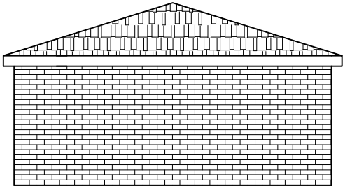
PROPOSED SIDE ELEVATIONS @1:100
