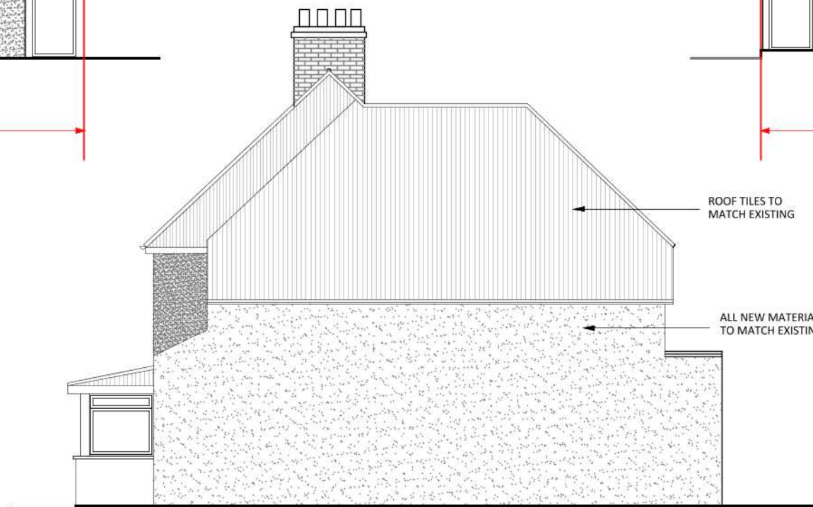
PROPOSED SIDE ELEVATION SOUTH EAST FACE
