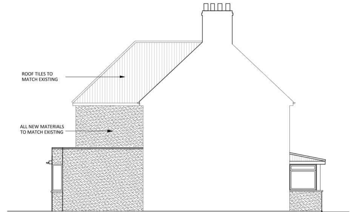
PROPOSED SIDE ELEVATION NORTH WEST FACE
