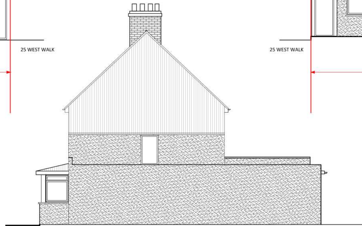
EXISTING SIDE ELEVATION SOUTH EAST FACE
