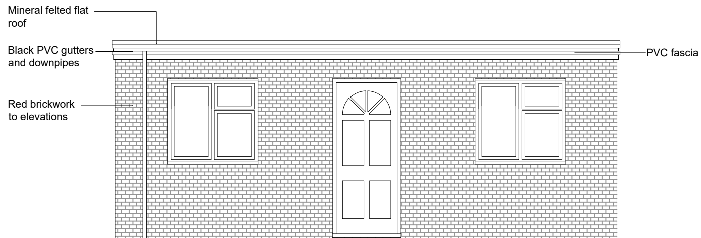
SOUTH ELEVATION
