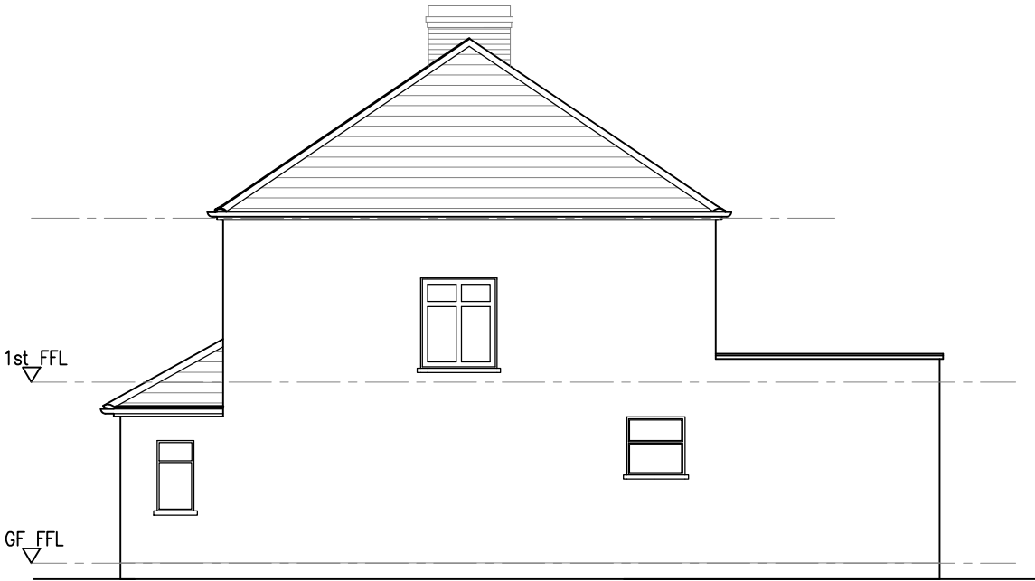
Side Elevation (facing no. 90)
