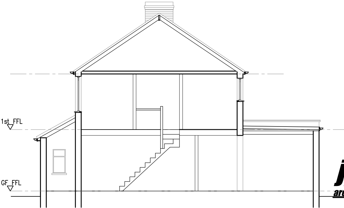
Section 1-1
