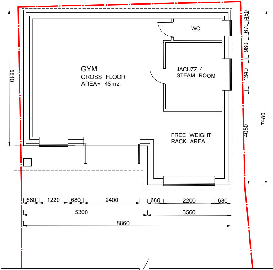
PROPOSED FLOOR PLAN SCALE 1:100
