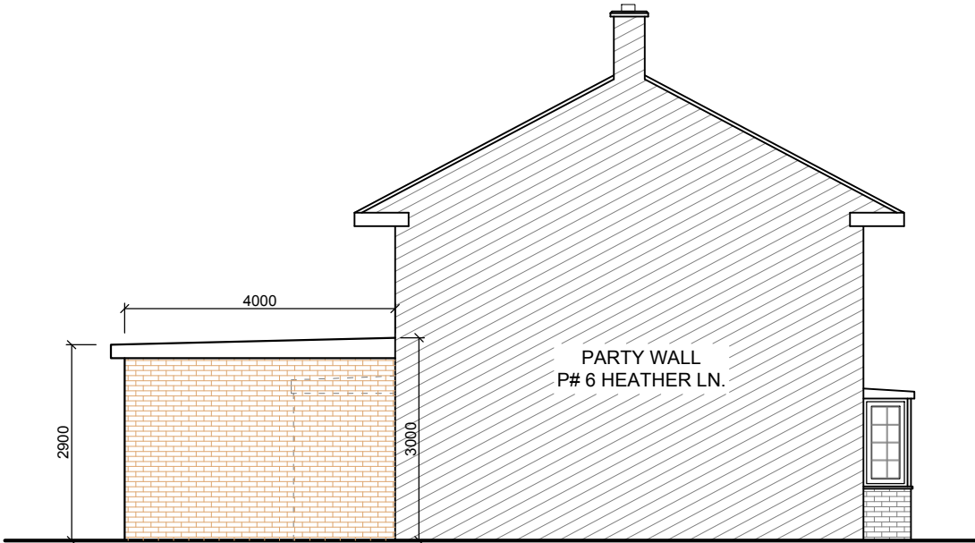
PROPOSED WEST SIDE(NO.6) ELEVATION SCALE= 1:100
