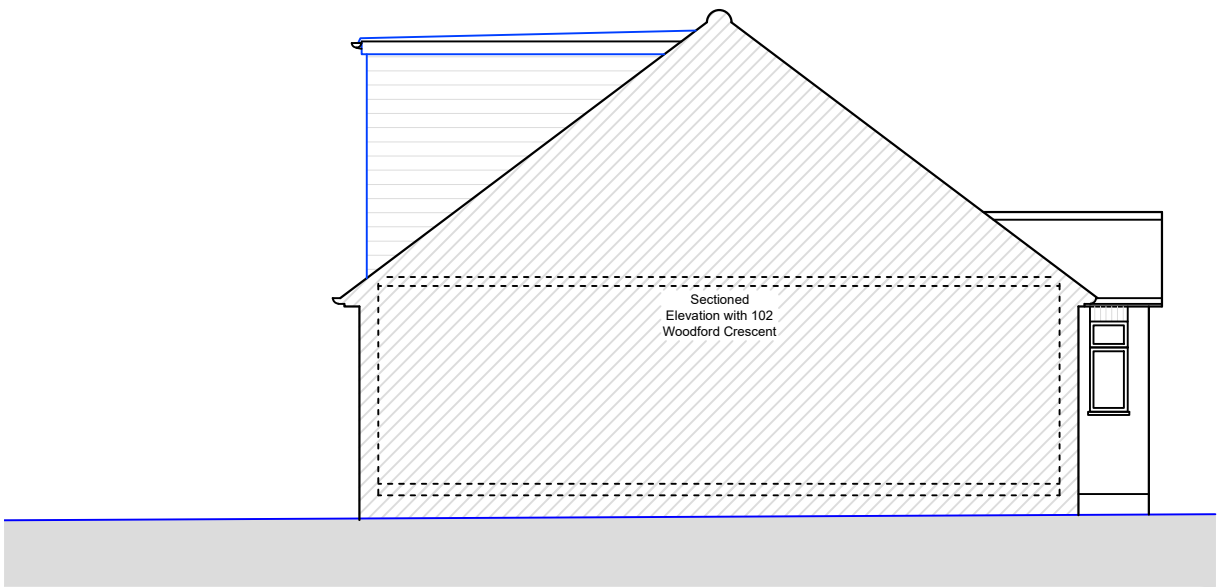
○ Side Elevation 2 1 : 1 0 0
