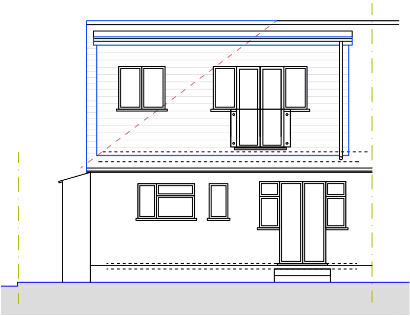
○ Rear Elevation 1 : 1 0 0
