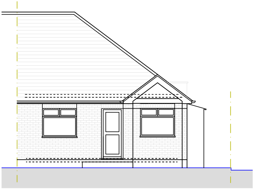
○ Front Elevation 1 : 1 0 0
