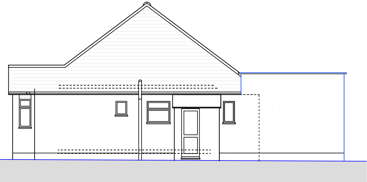
○ Side Elevation 1 1 : 1 0 0
