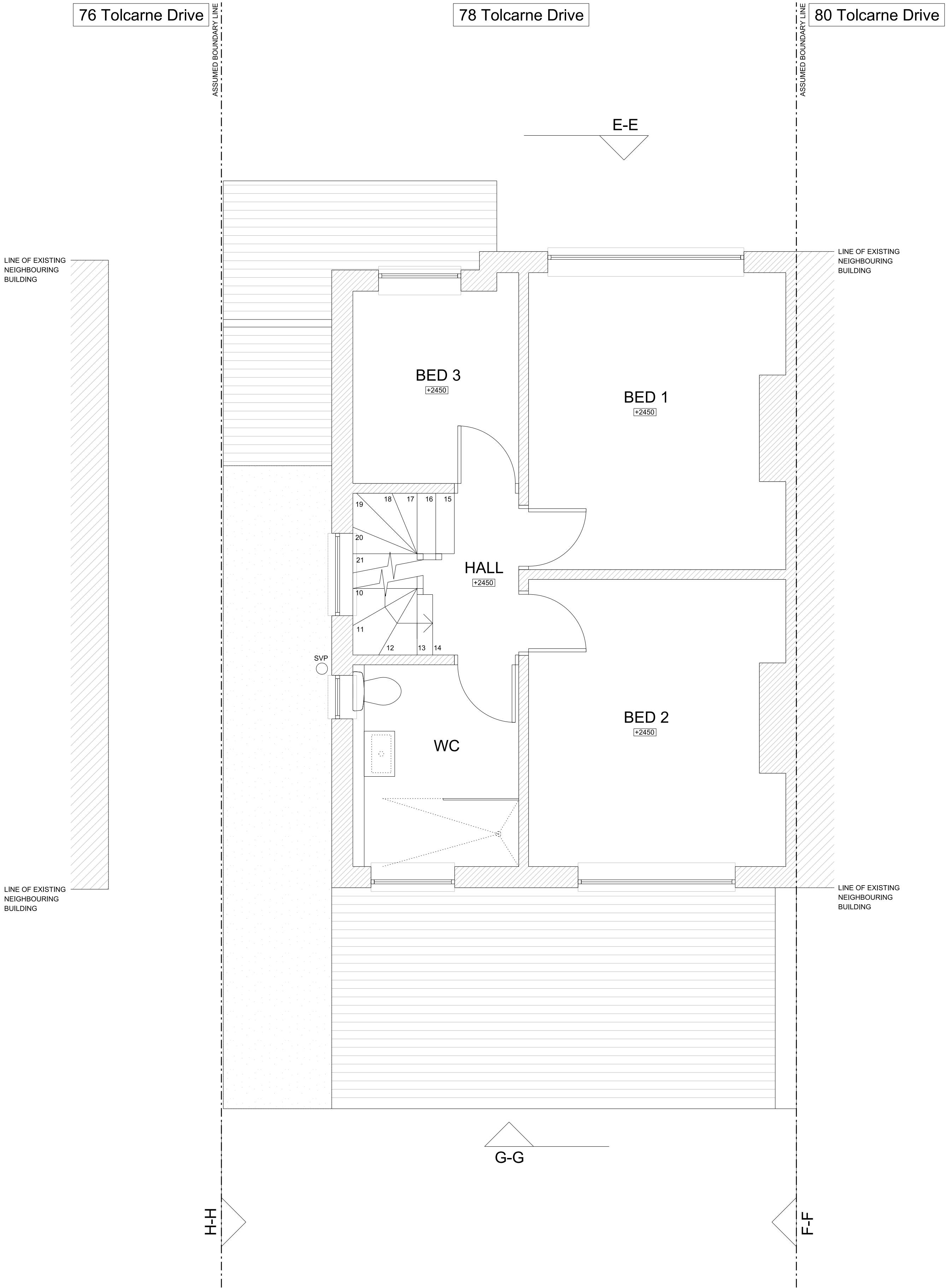
2. PROPOSED FIRST FLOOR PLAN
