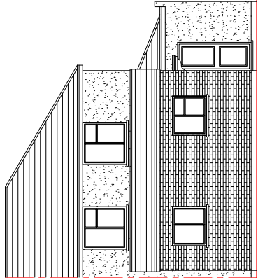
Proposed Rear Elevation Scale 1:100
