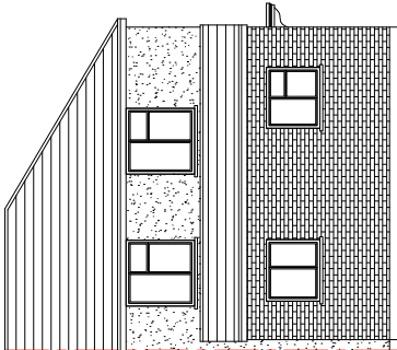
Existing Rear Elevation Scale 1:100
