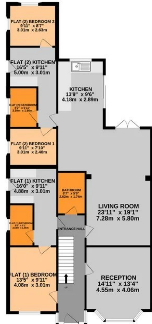
GROUND FLOOR 1475 sq.ft. (137.0 sq.m.) approx.
