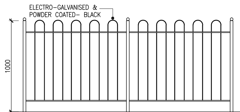
METAL RAILINGS FENCE DETAIL
