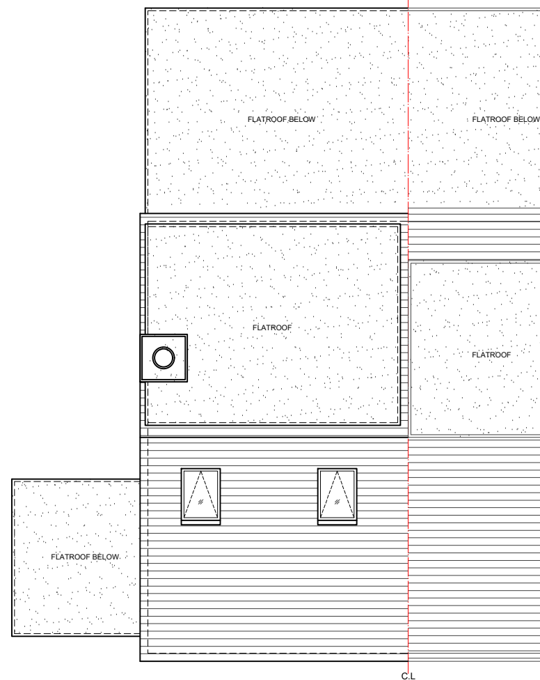
04 - ROOF PLAN
