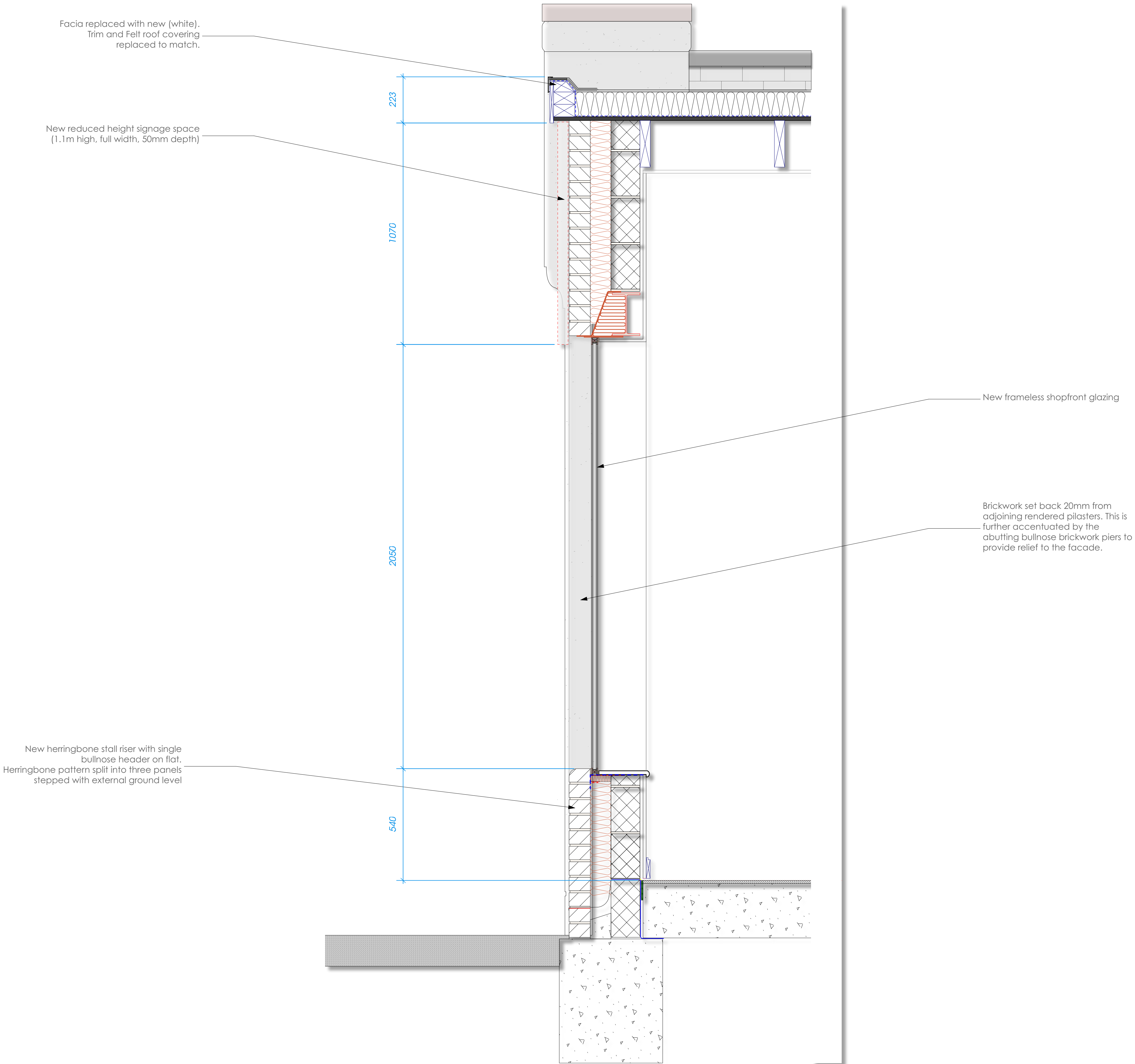
1 2204 No. 65 Shop front Section Scale: 1:10
