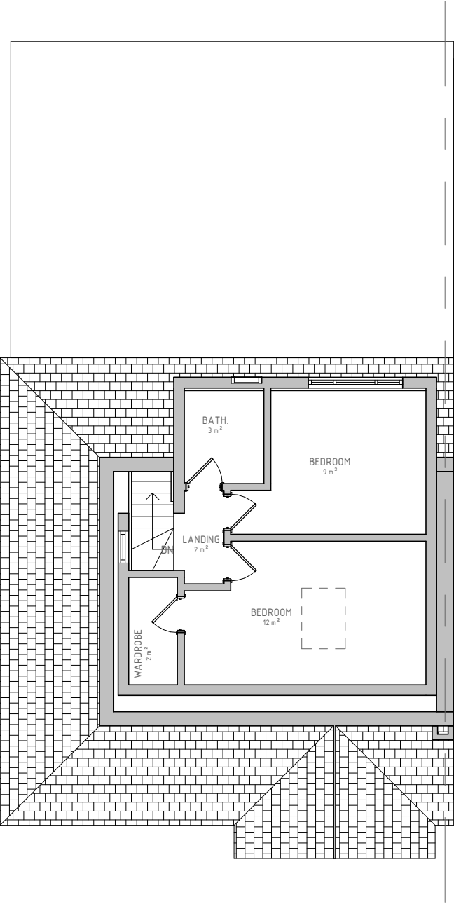
03/102 - EXISTING FIRST FLOOR PLAN 1 : 100
