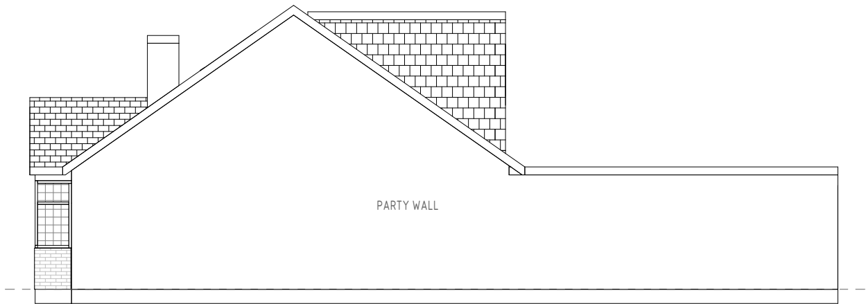
04/204 - EXISTING RIGHT ELEVATION 1 : 100
