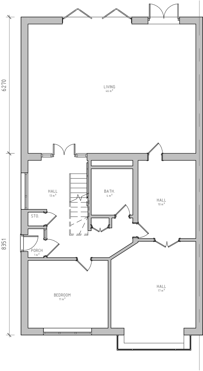
03/101 - EXISTING GROUND FLOOR PLAN 1 : 100
