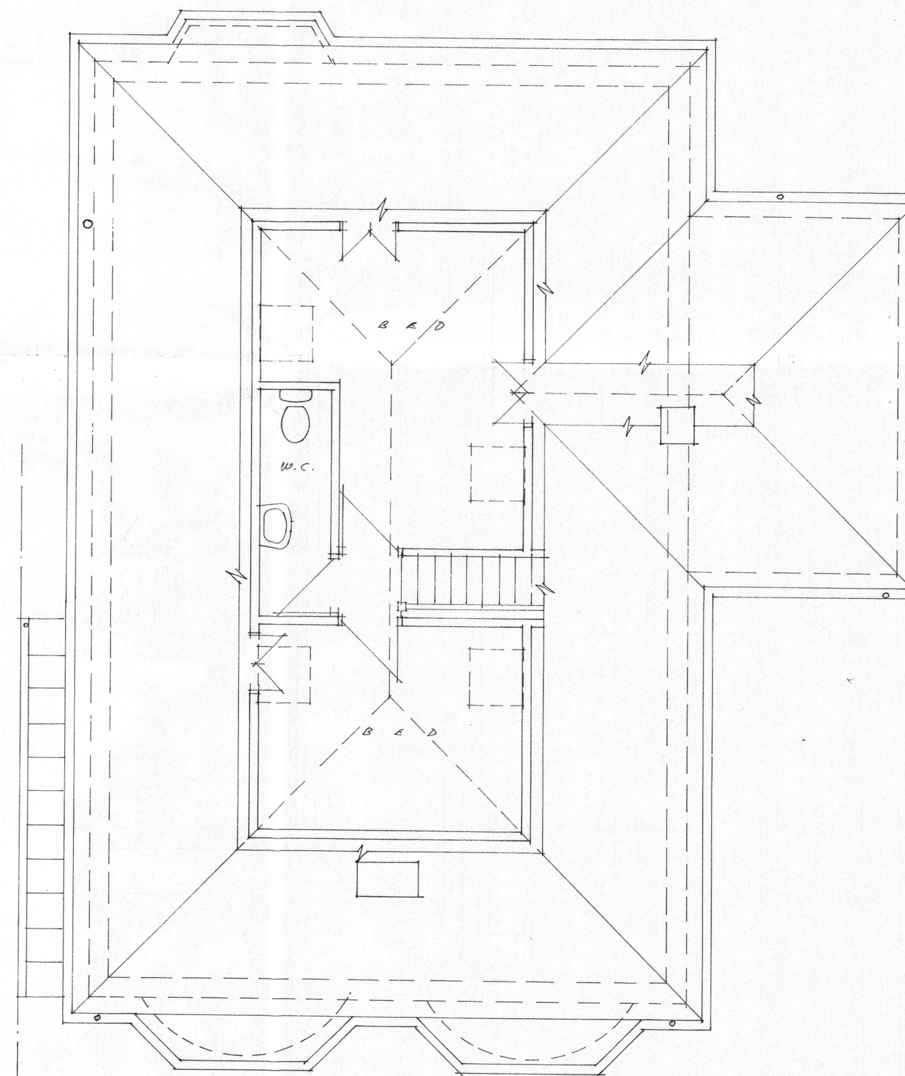
FIRST FLOOR
