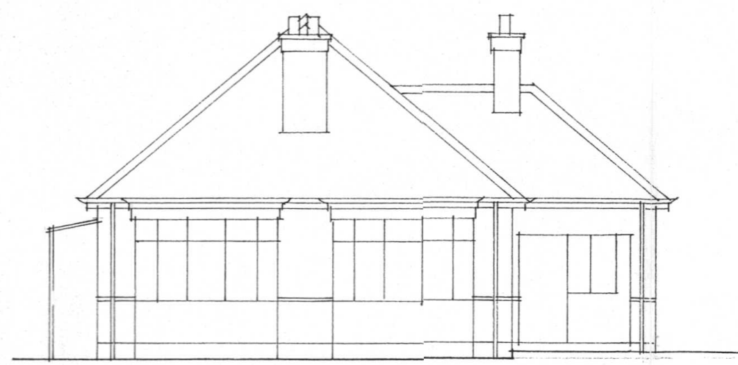
FRONT
