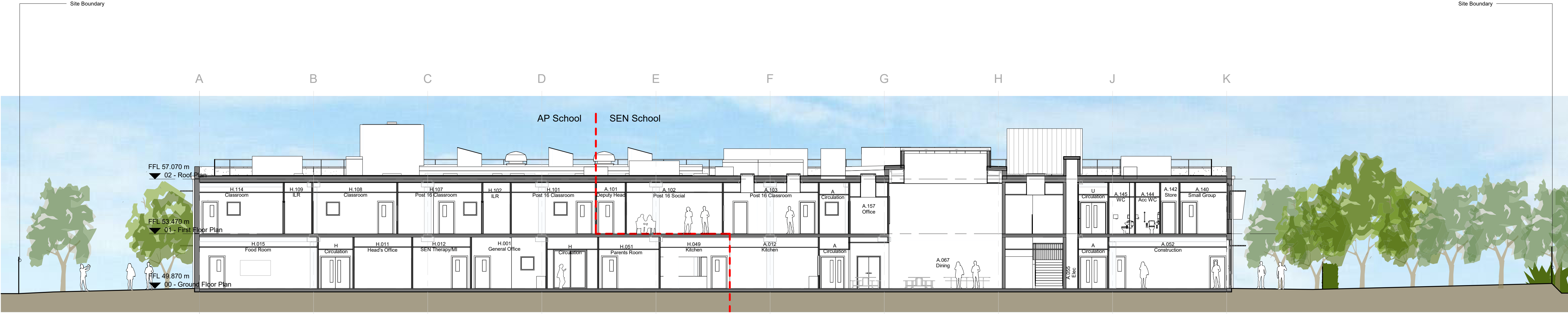
1 Proposed long section through kitchens and SEN dining SCALE 1 : 125
