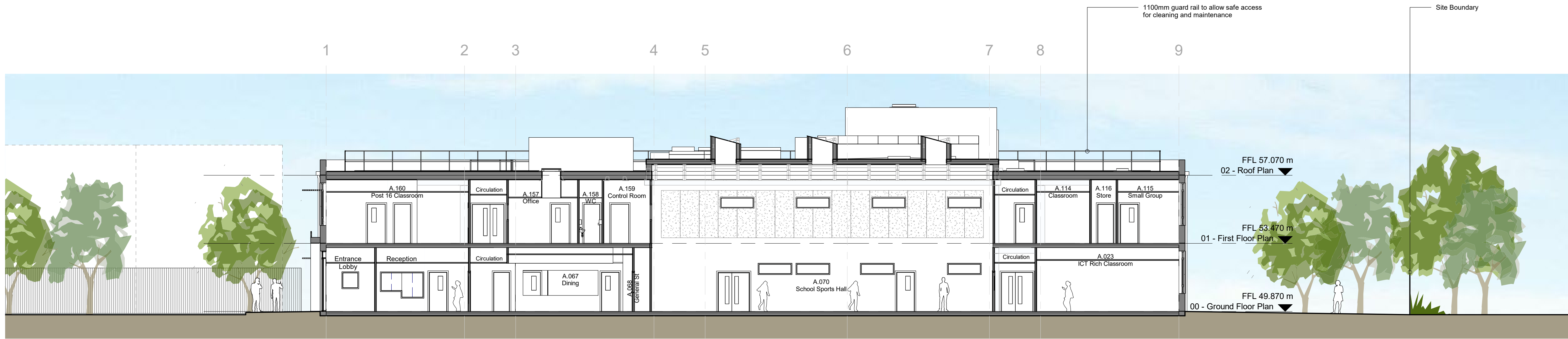
2 Proposed Cross Section through SEN entrance SCALE 1 : 125
