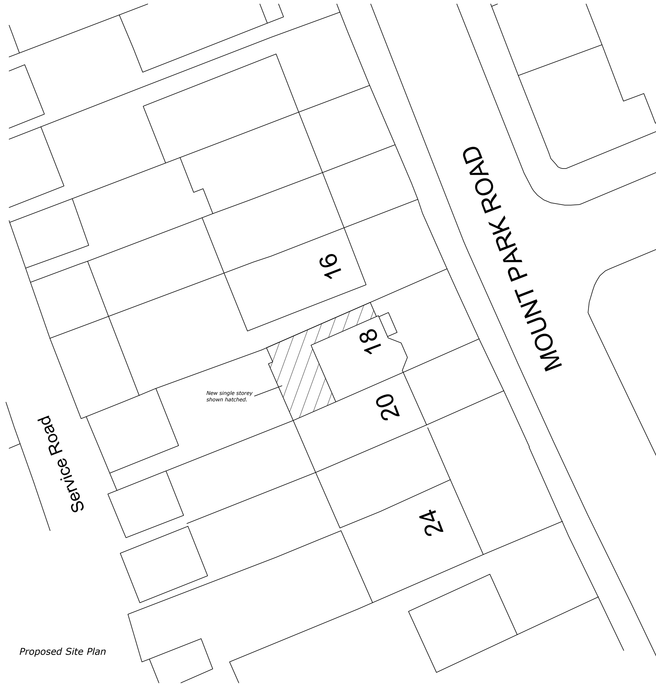
Existing & Proposed Site Plans
