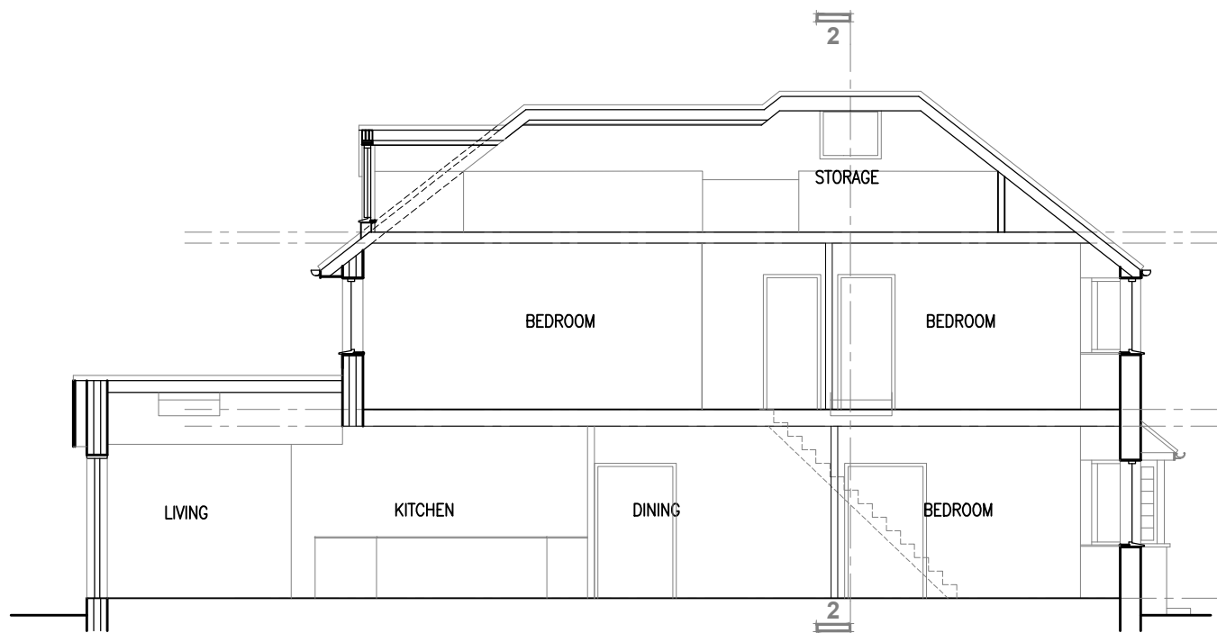
SECTION 1-1
