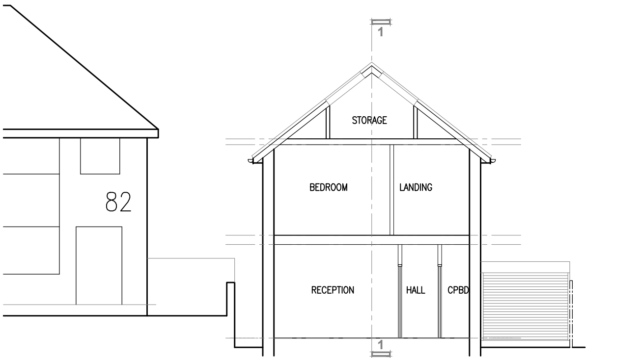
SECTION 2-2
