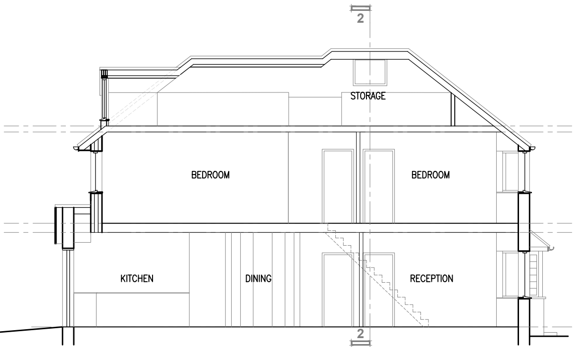
SECTION 1-1
