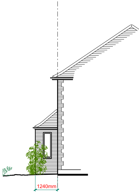
04 PROPOSED SIDE ELEVATION SCALE 1:100
