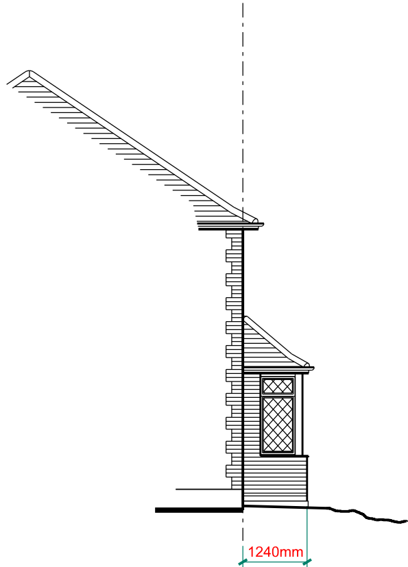
01 EXISTING SIDE ELEVATION SCALE 1:100
