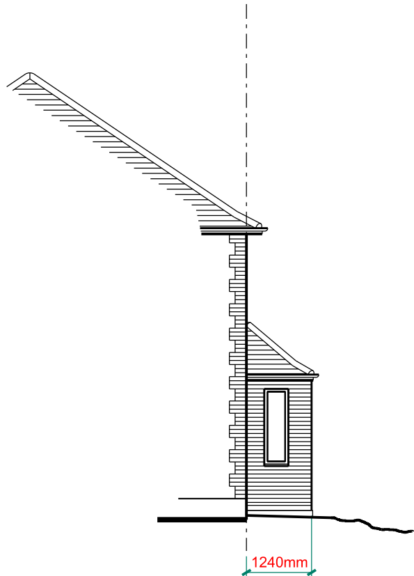
02 PROPOSED SIDE ELEVATION SCALE 1:100
