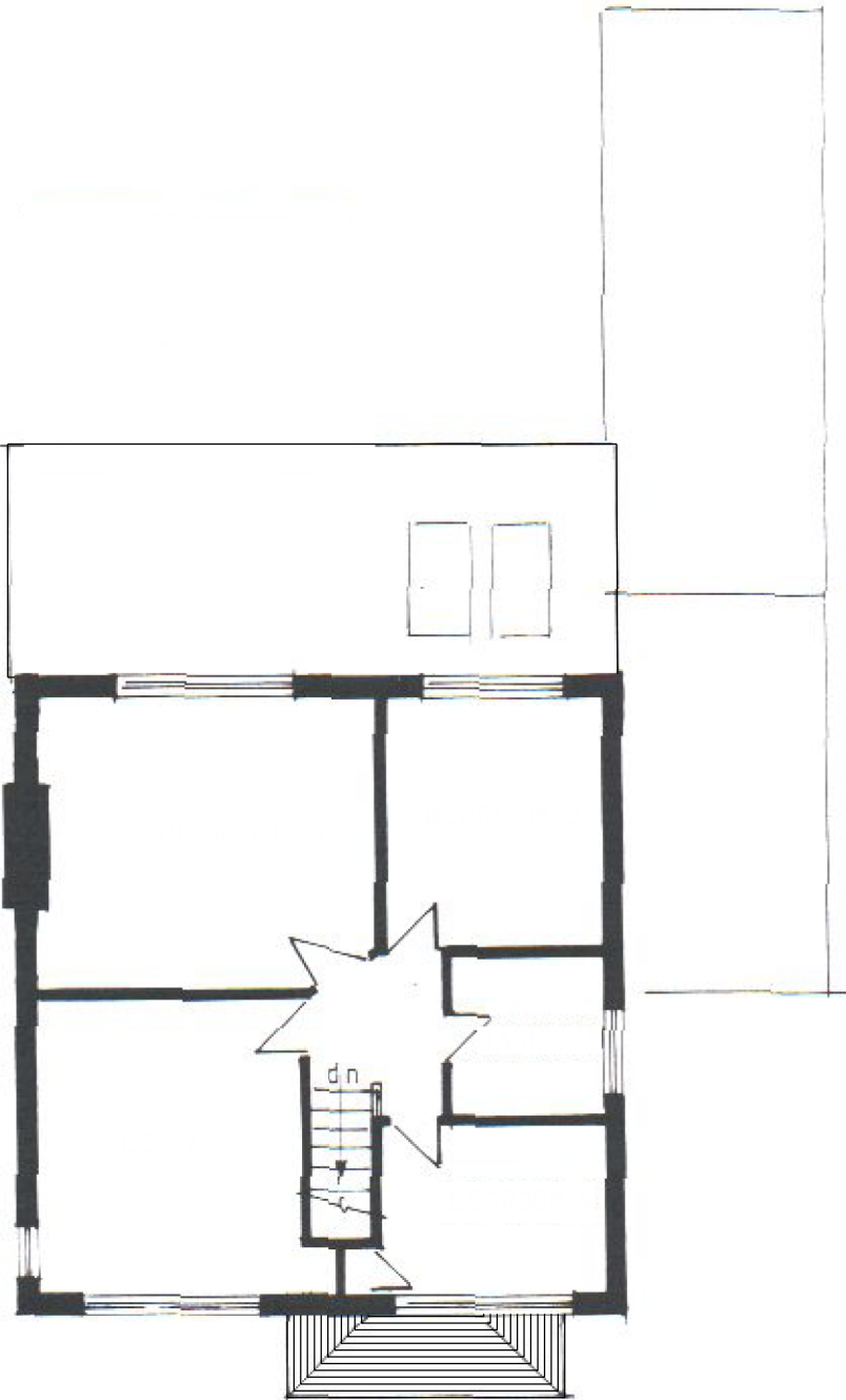
01 EXISTING FIRST FLOOR PLAN SCALE 1:100
