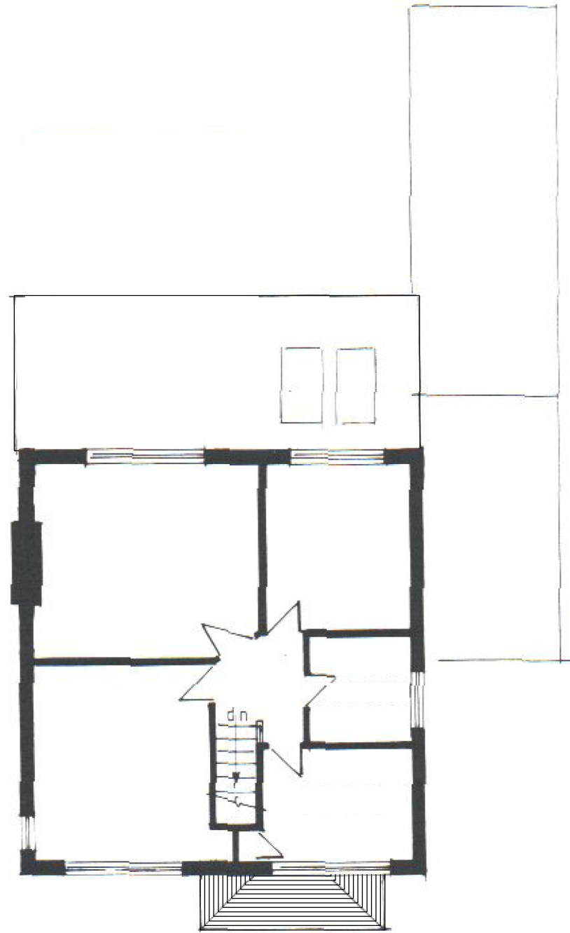
01 EXISTING FIRST FLOOR PLAN SCALE 1:100
