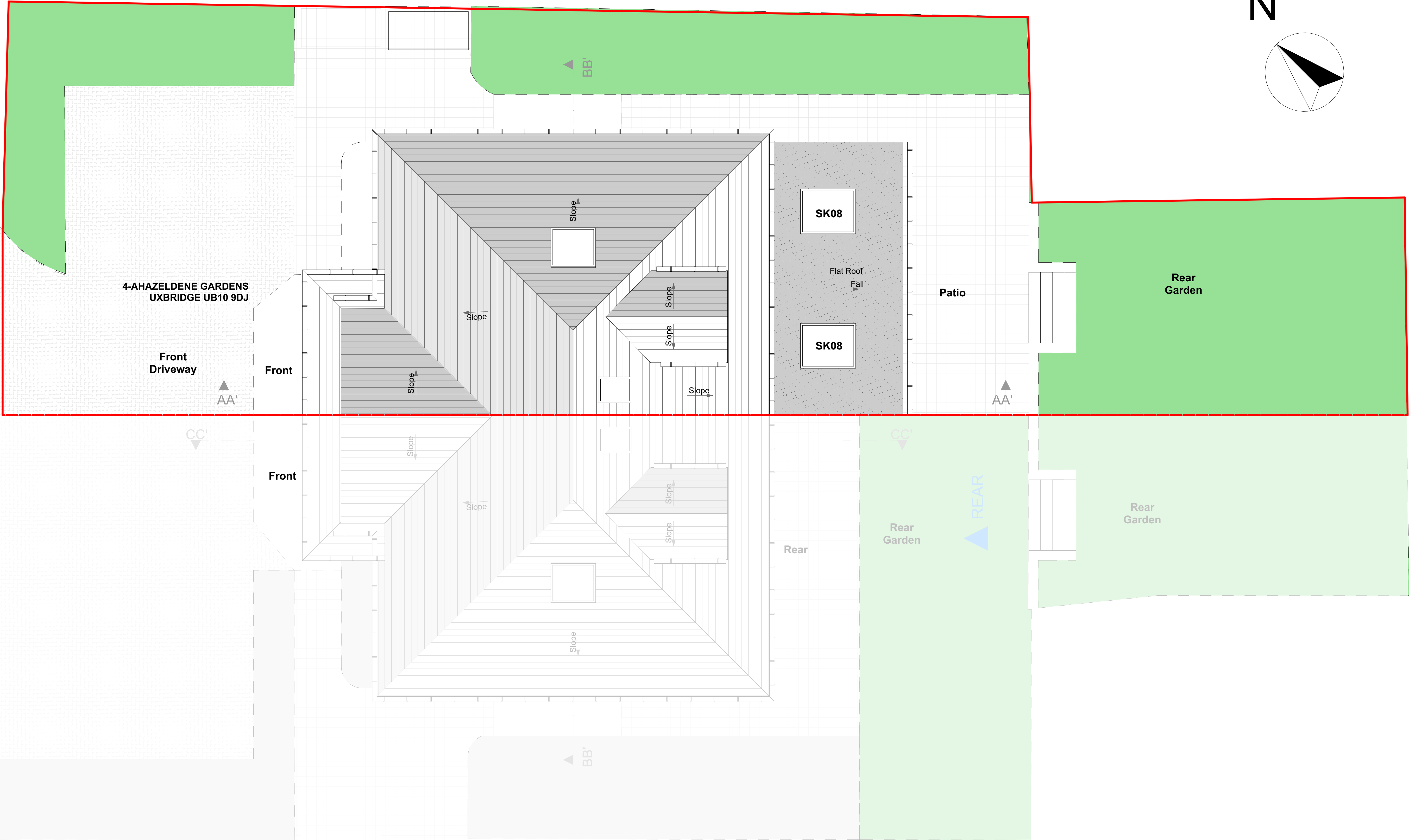
Proposed Roof Plan 1:50
